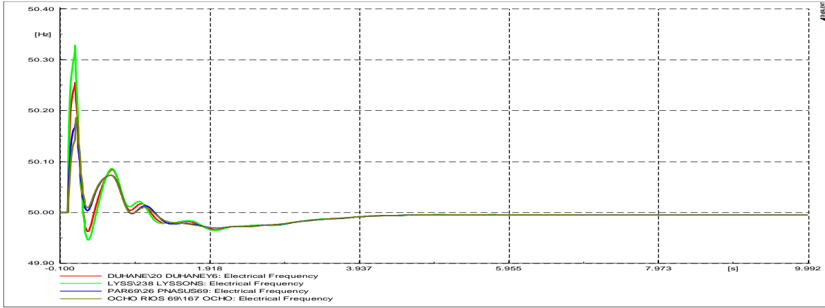
Figure 7.15: Bus Frequencies
