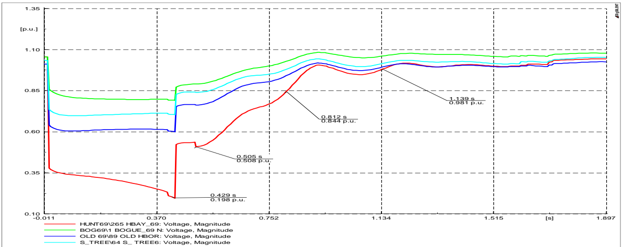
Figure 7.41: Bus voltages
