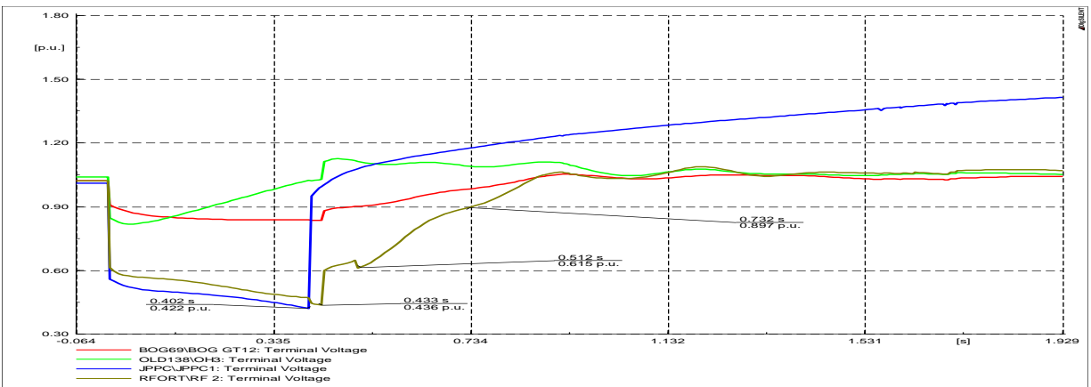
Figure 7.37: Generator Terminal Voltages
