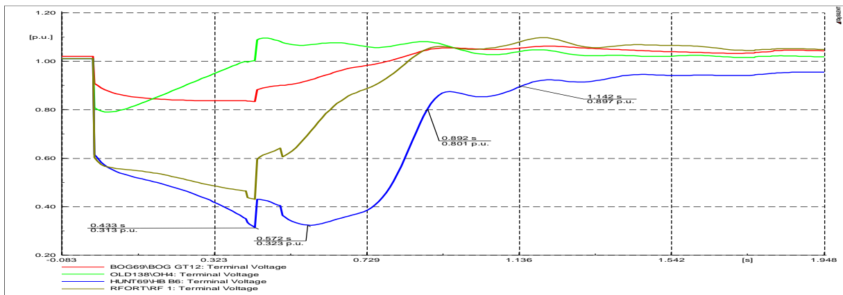
Figure 7.31: Generator Terminal Voltages
