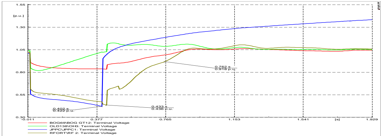
Figure 7.30: Generator Terminal Voltages
