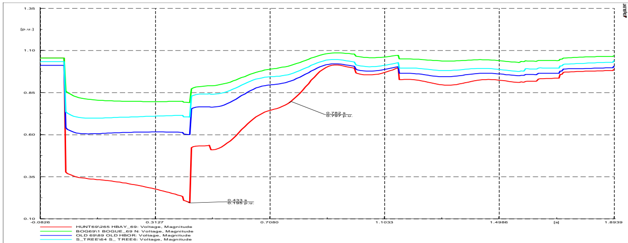
Figure 7.48: Bus Voltages
