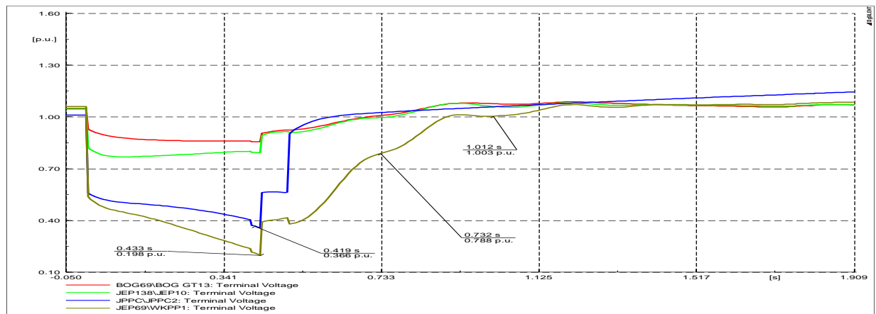
Figure 7.32: Generator Terminal Voltages
