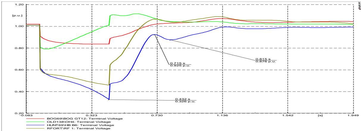
Figure 7.24: Generator Terminal Voltages
