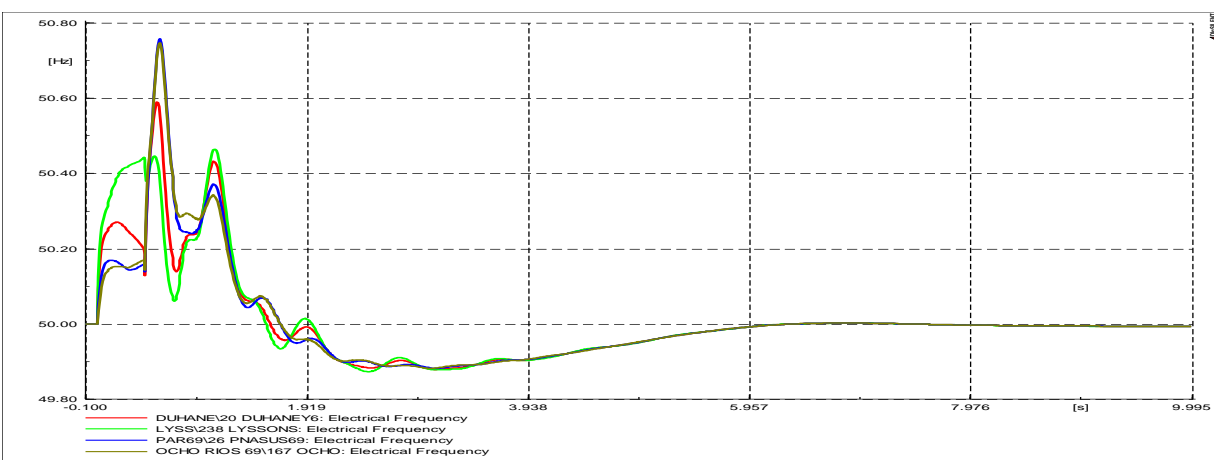
Figure 7.29: Bus frequencies
