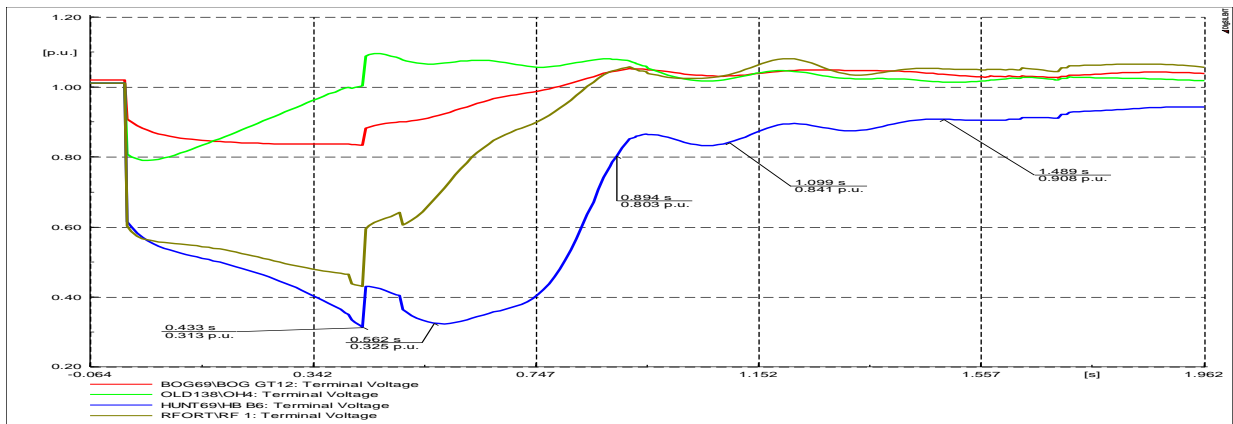
Figure 7.38: Generator Terminal Voltages
