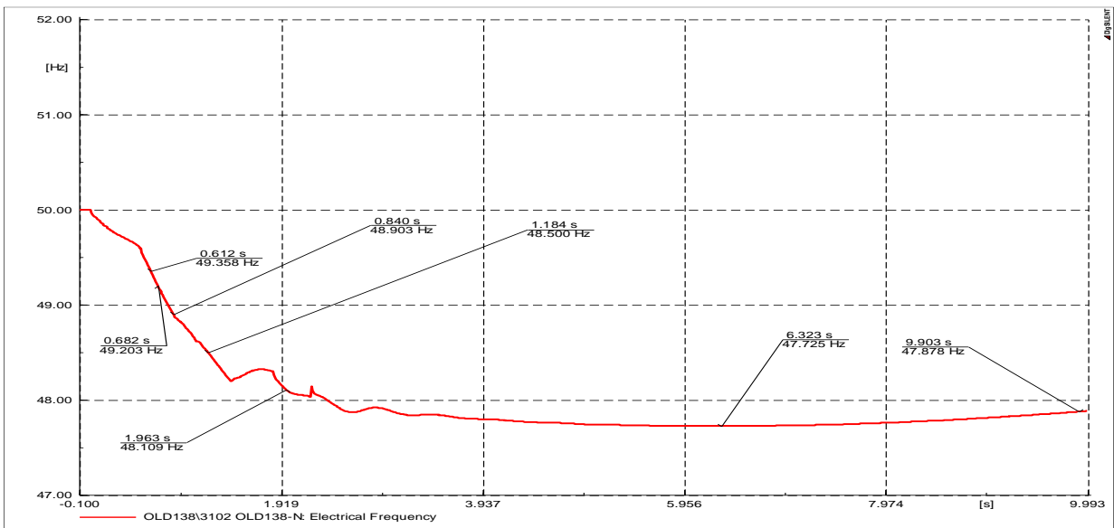
Figure 7.55: Bus Frequencies
