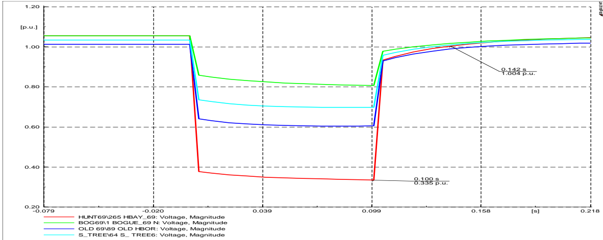
Figure 7.12: Bus Voltages
