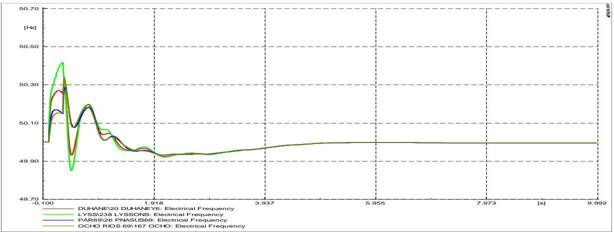
Figure 7.22: Bus Frequencies
