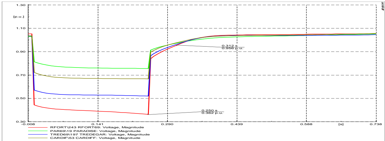
Figure 7.21: Bus Voltages
