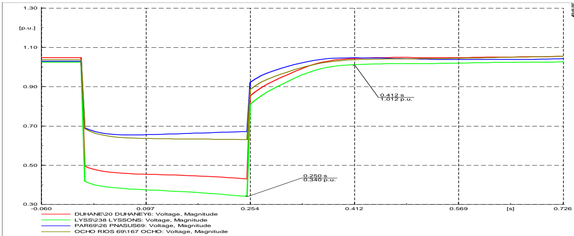
Figure 7.20: Bus Voltages
