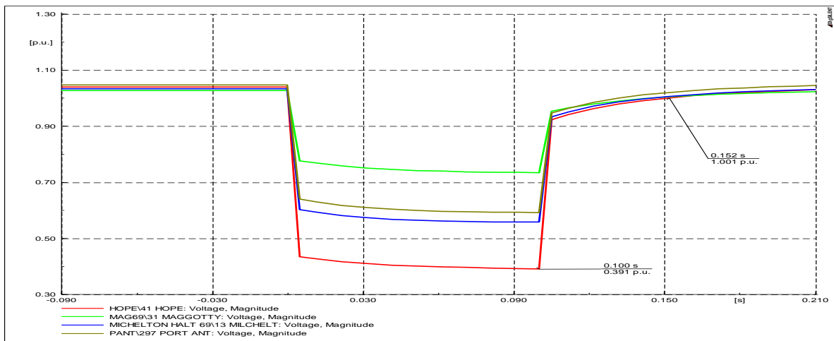
Figure 7.14: Bus Voltages
