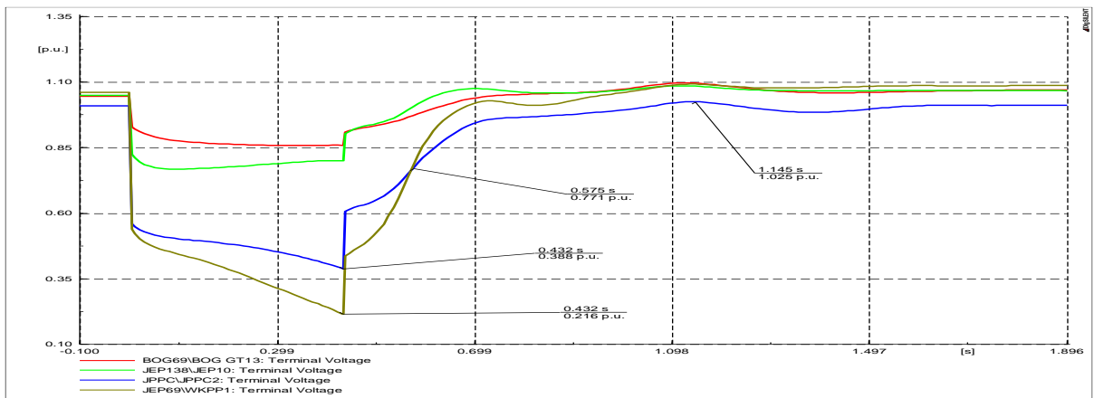
Figure 7.25: Generator Terminal Voltages
