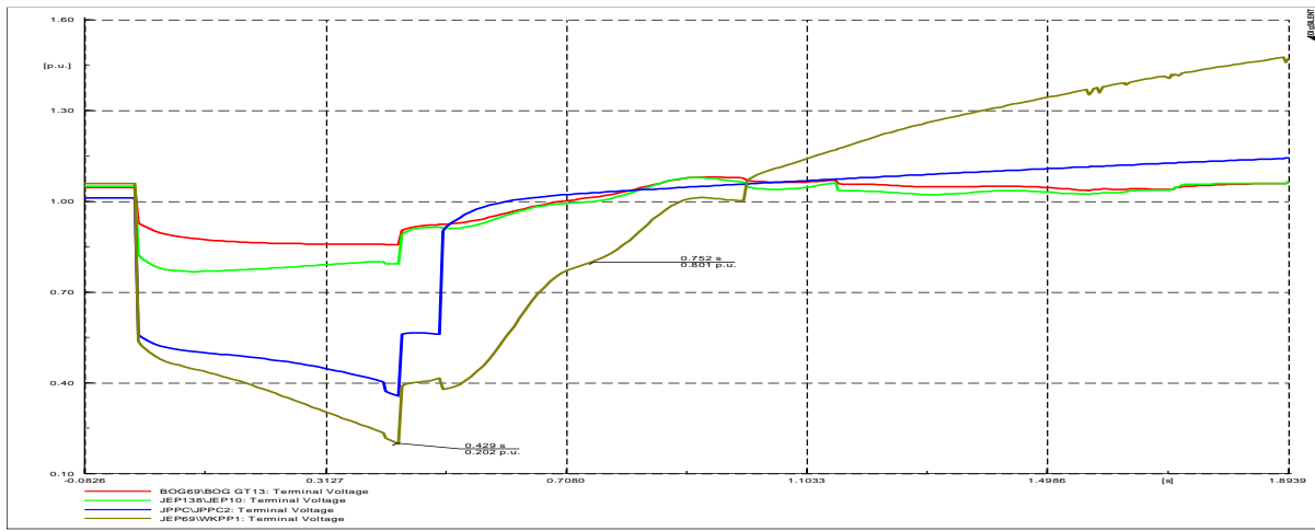
Figure 7.46: Generator Terminal Voltages
