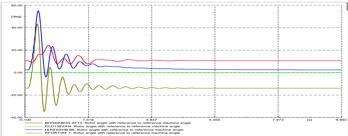
Figure 7.17: Generator Rotor Angles
