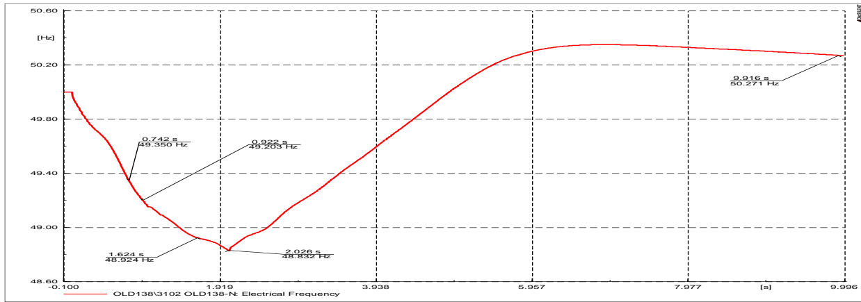
Figure 7.52: Bus Frequencies
