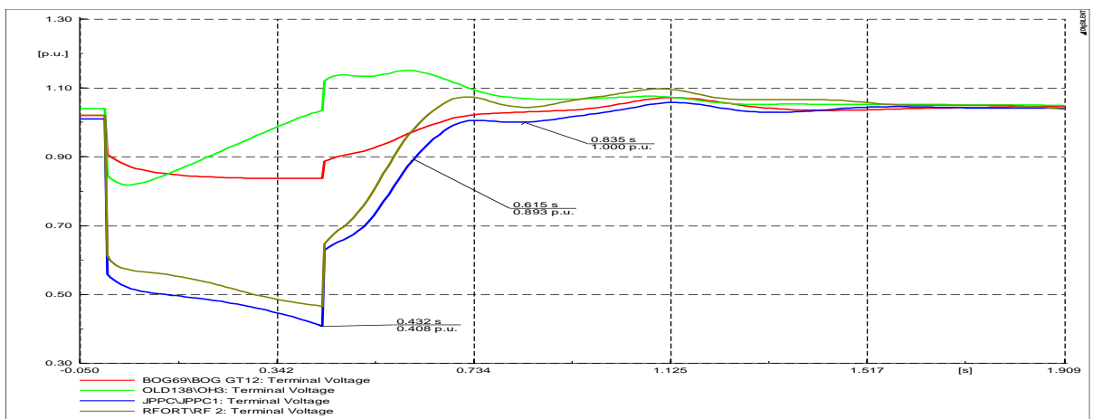
Figure 7.26: Bus Voltages
