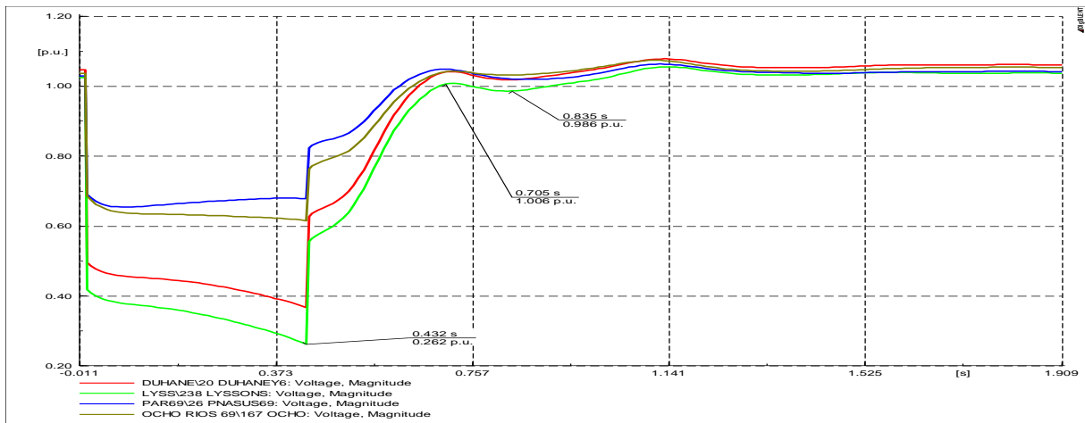
Figure 7.27: Bus voltages
