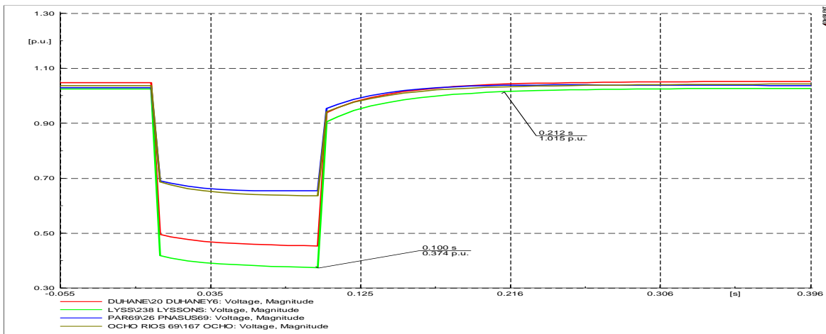
Figure 7.13: Bus Voltages
