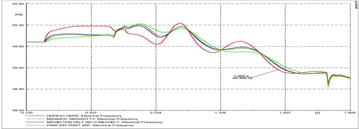
Figure 7.36: Bus Frequencies
