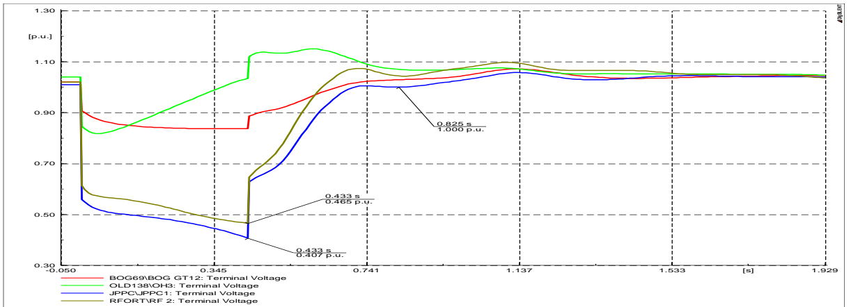
Figure 7.23: Generator Terminal Voltages
