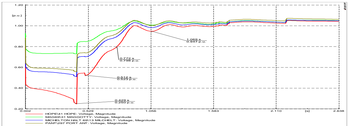
Figure 7.43: Bus Voltages
