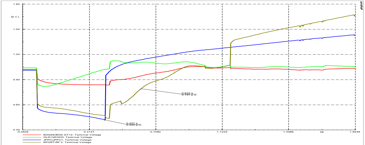
Figure 7.45: Generator Terminal Voltages
