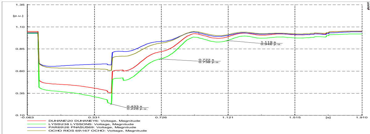
Figure 7.42: Bus Voltages
