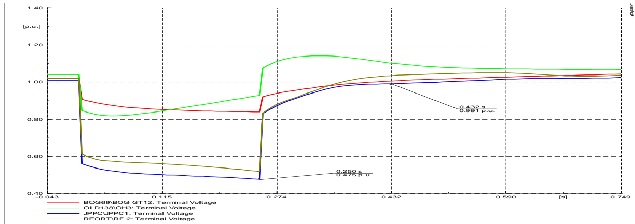
Figure 7.16: Generator Terminal Voltages
