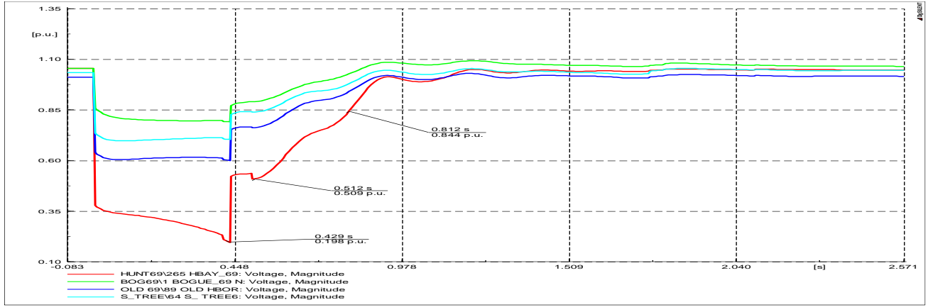
Figure 7.33: Bus Voltages
