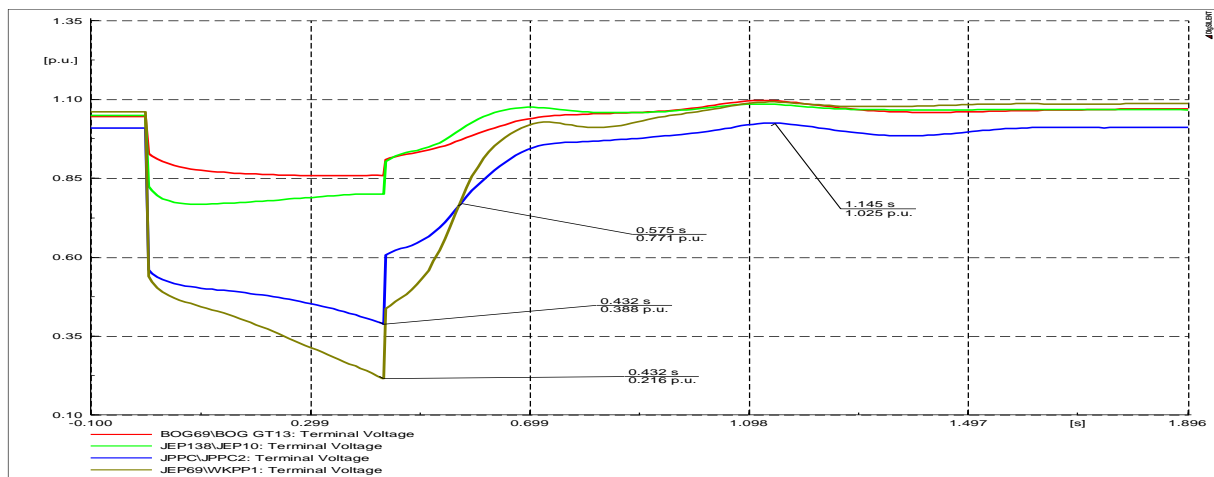
Figure 7.28: Bus Voltages
