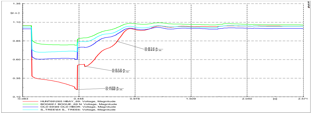
Figure 7.34: Bus Voltages
