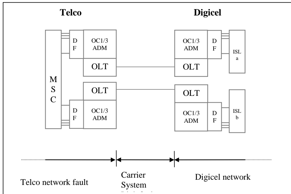
2.5.2.2 Figure 4. Fault Classification in Network Segments
