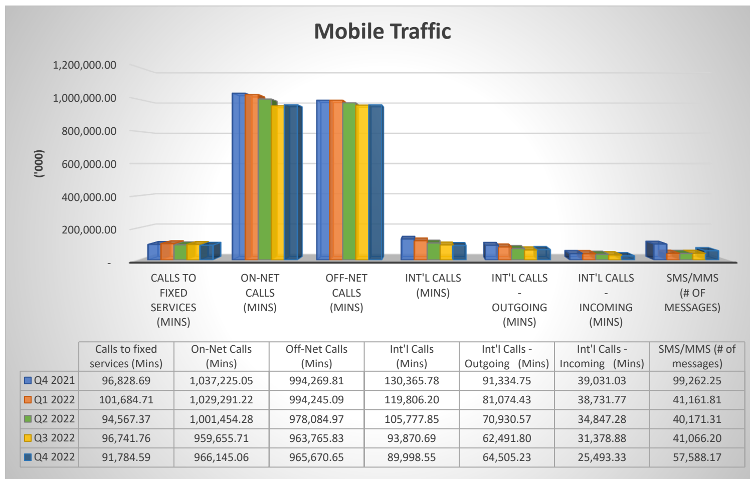
Figure 6: Mobile Traffic
